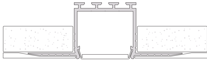
Drywall Installation Example
