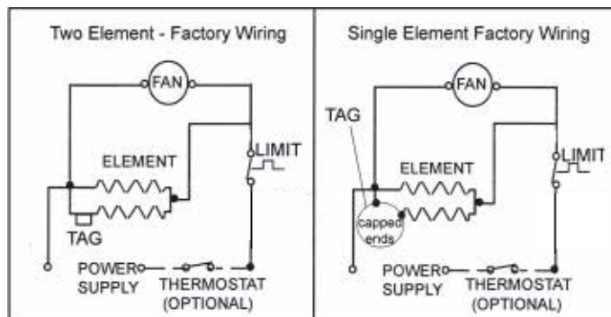
Wiring Diagram
