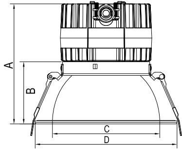
Round Reflector
