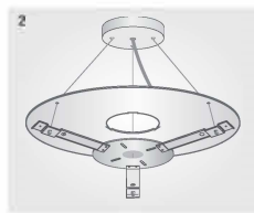
Step 2 Put electrical cord and decorative nut on the electrical cable as shown. Then insert end of the steel wire into the ceiling base as shown and put the electric cable through the central hole.
