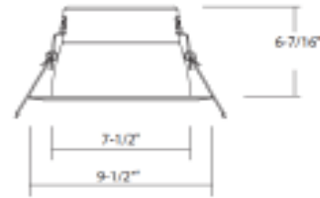
Ceiling Cut-out : 8-1/4"
