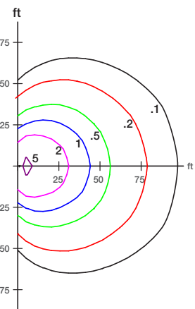
80W luminaire mounted at 25ft
