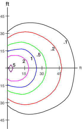
29W luminaire mounted at 15ft
