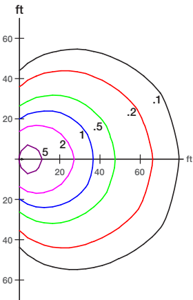
60W luminaire mounted at 20ft
